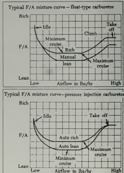
FIGURE 3-1. Fuel/air mixture curves.
